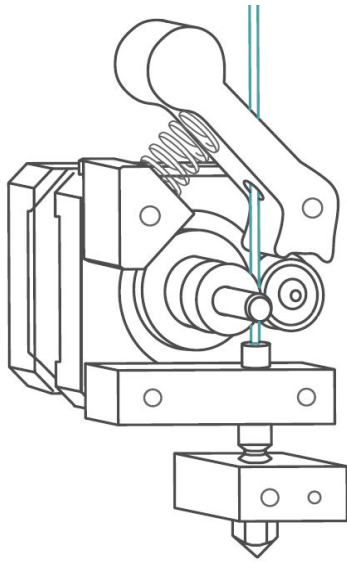
Figure 2: Extruder
